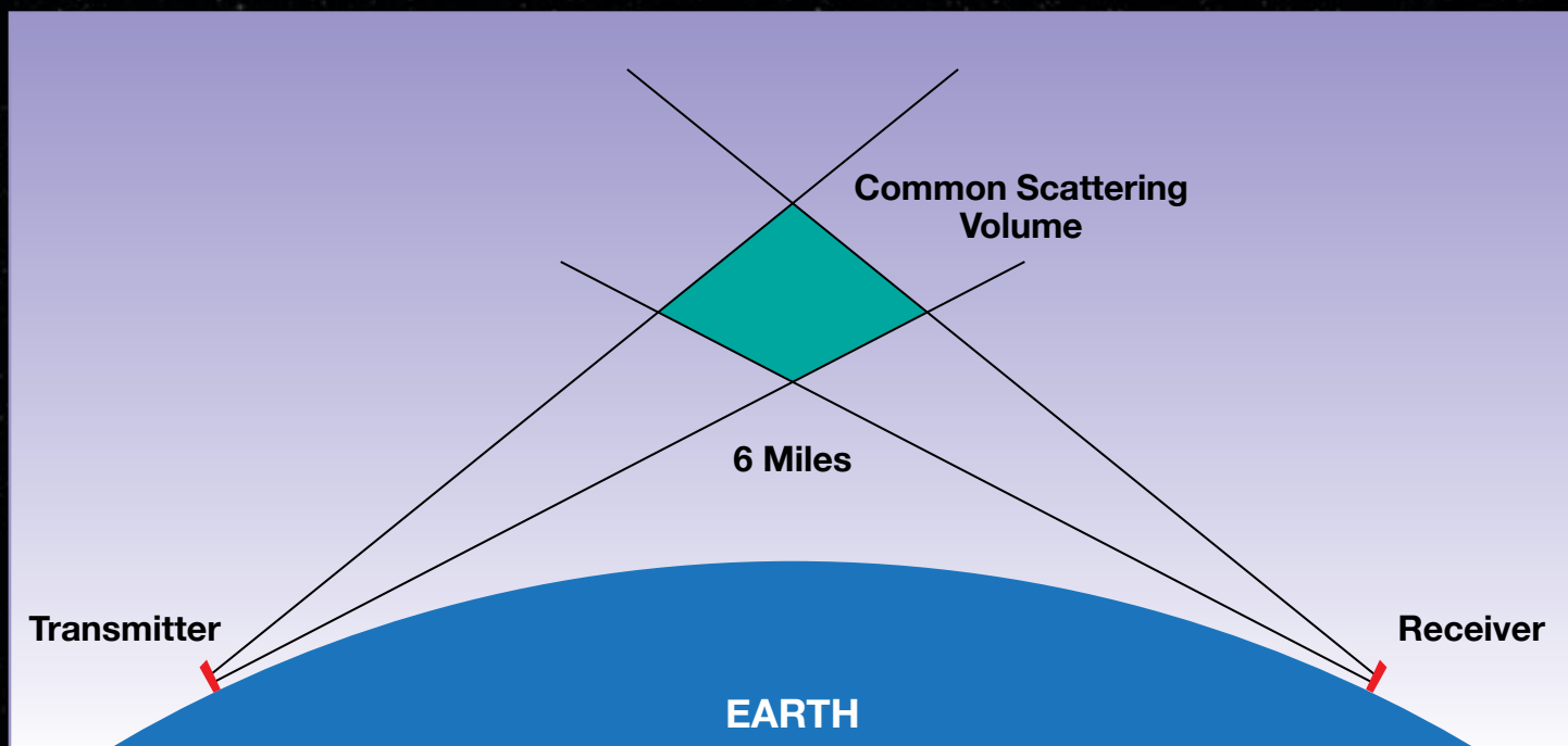
This drawing illustrates how troposcatter communications can carry voice and data at beyond-line-of-sight distances.
